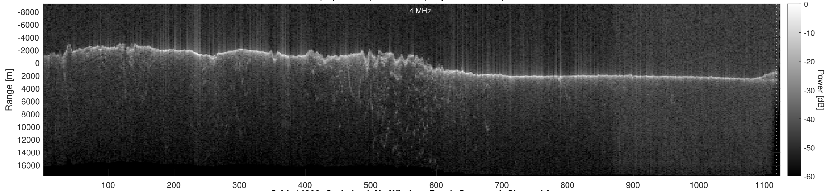
Orbit 14303, Optimized, No Window, Depth-Corrected, Channel 2
