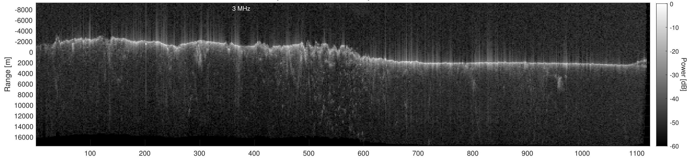
Orbit 14303, Depth-Corrected Cluttergram
