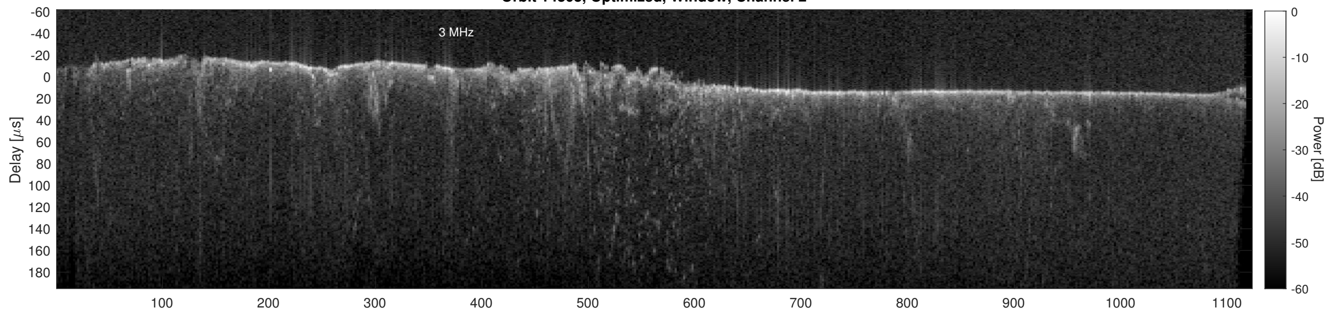
Orbit 14303, Cluttergram
