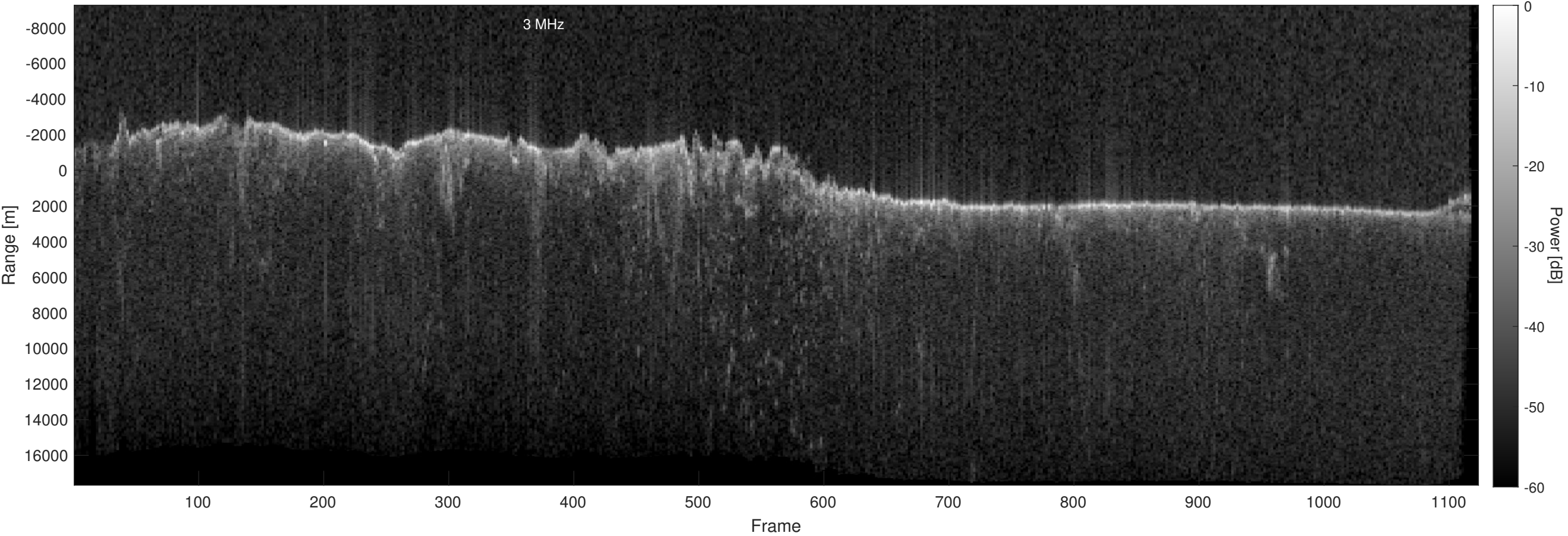
Orbit 14303, Optimized, Window, Depth-Corrected, Channel 2
