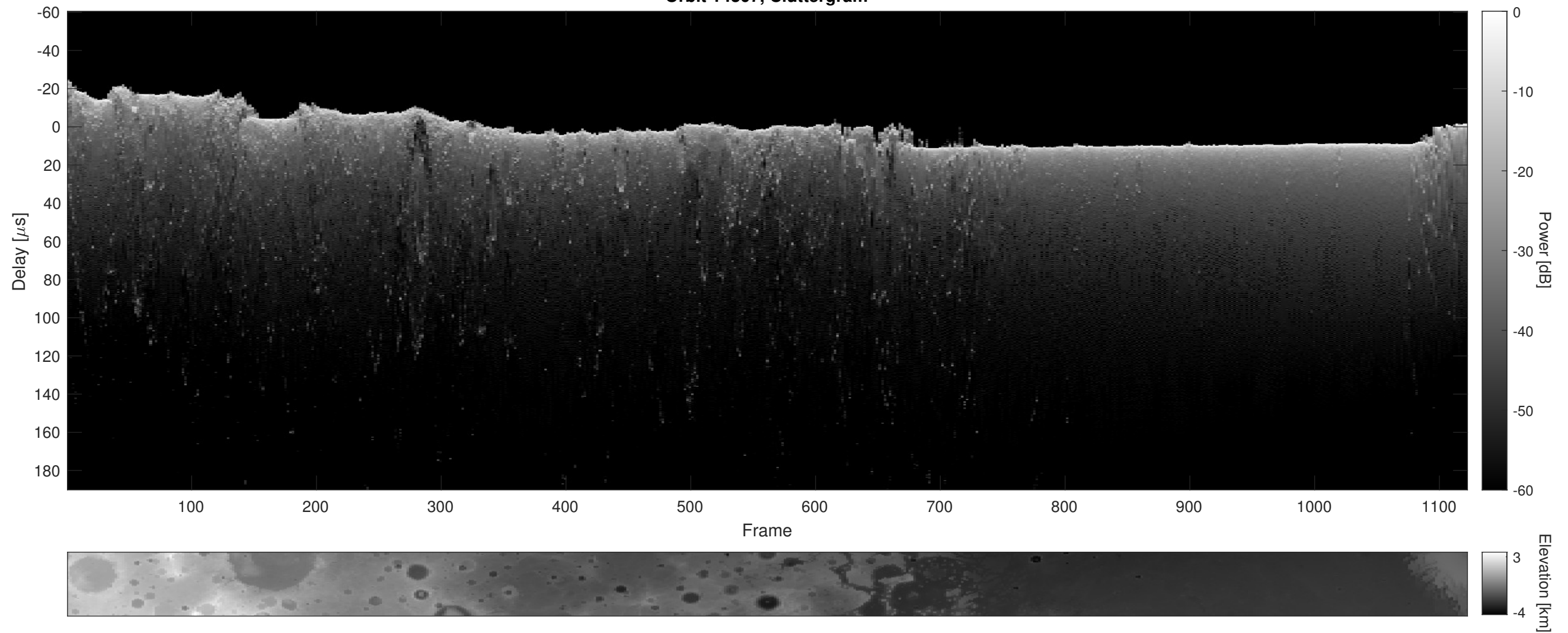
Orbit 14307, Cluttergram
