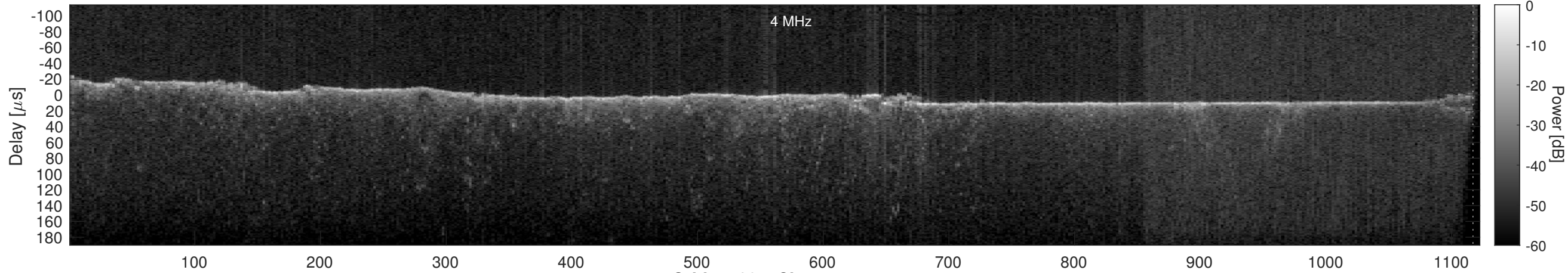
Orbit 14307, Cluttergram
