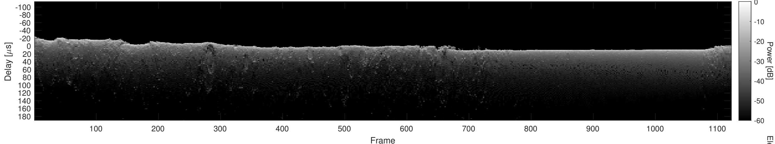
Orbit 14307, Cluttergram
