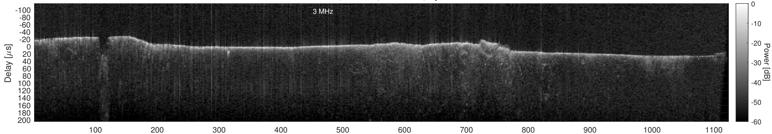
Orbit 14308, Cluttergram
