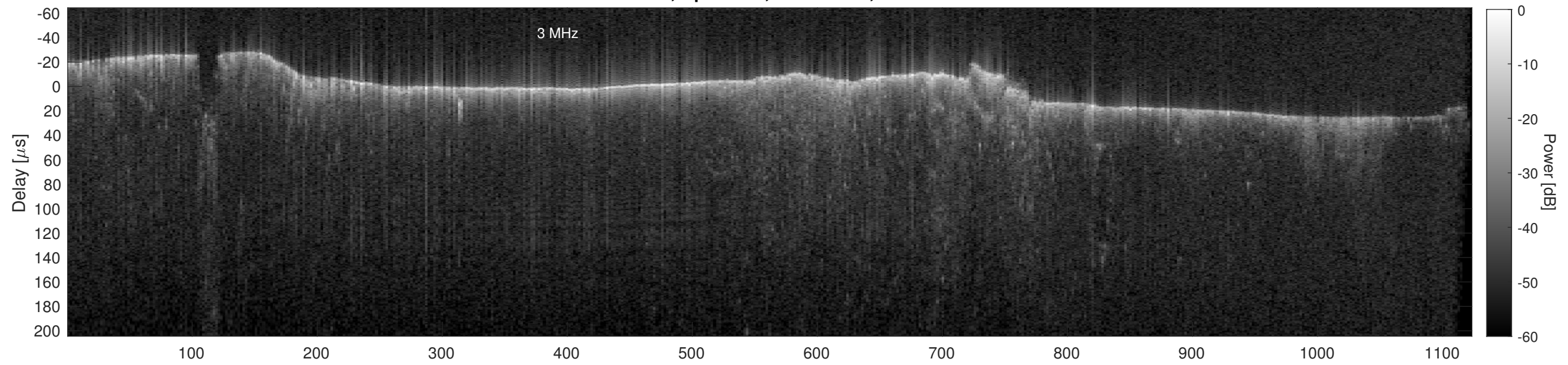
Orbit 14308, Cluttergram
