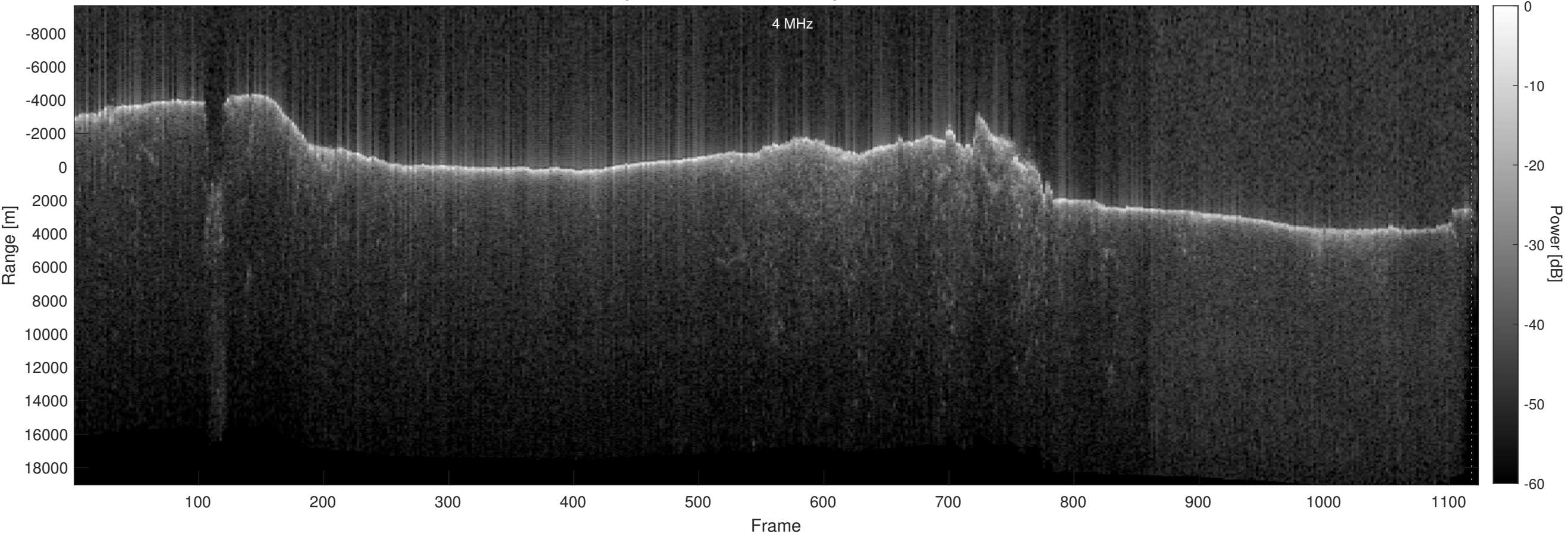
Orbit 14308, Optimized, No Window, Depth-Corrected, Channel 2
