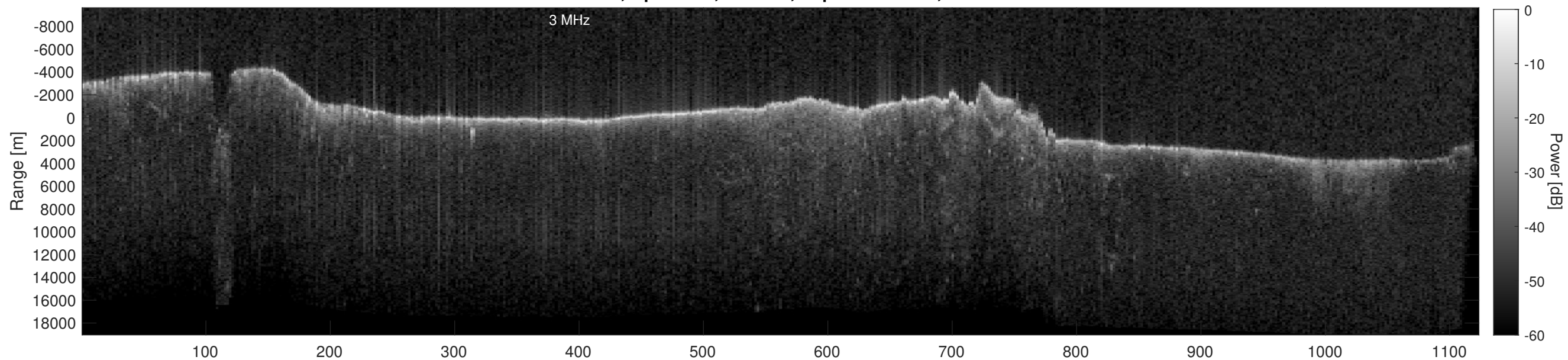
Orbit 14308, Depth-Corrected Cluttergram
