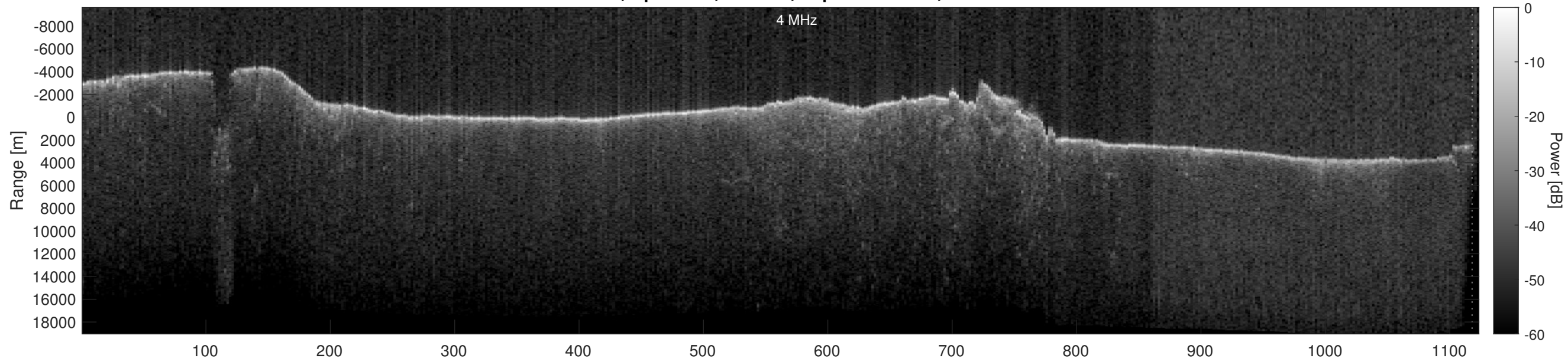
Orbit 14308, Optimized, Window, Depth-Corrected, Channel 2
