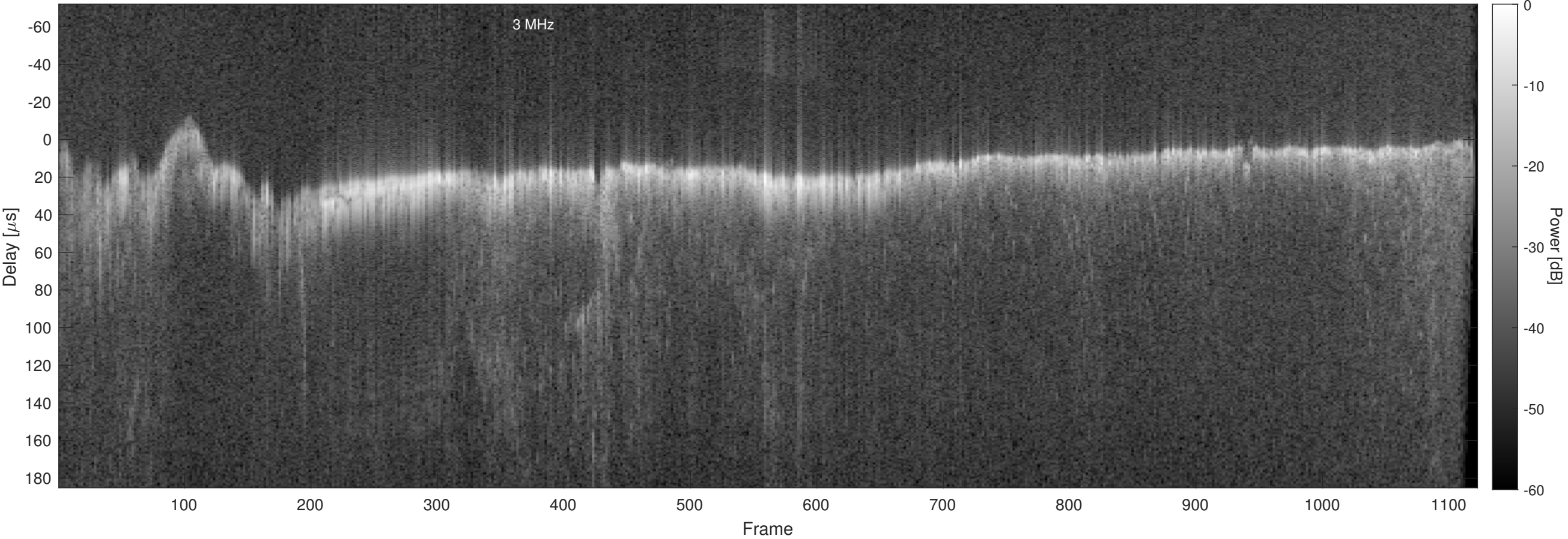
Orbit 14309, Chapman, No Window, Channel 2
