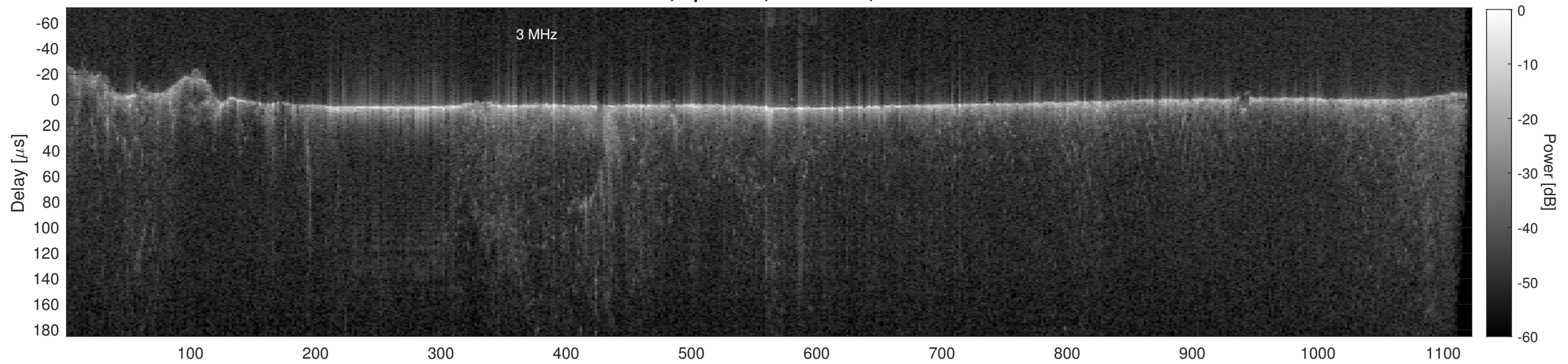
Orbit 14309, Cluttergram
