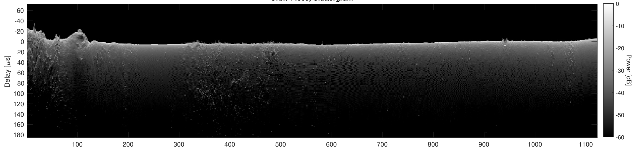
Orbit 14309, Cluttergram
