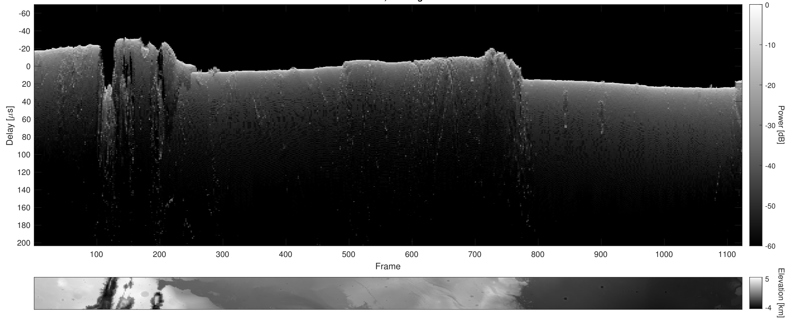
Orbit 14315, Cluttergram
