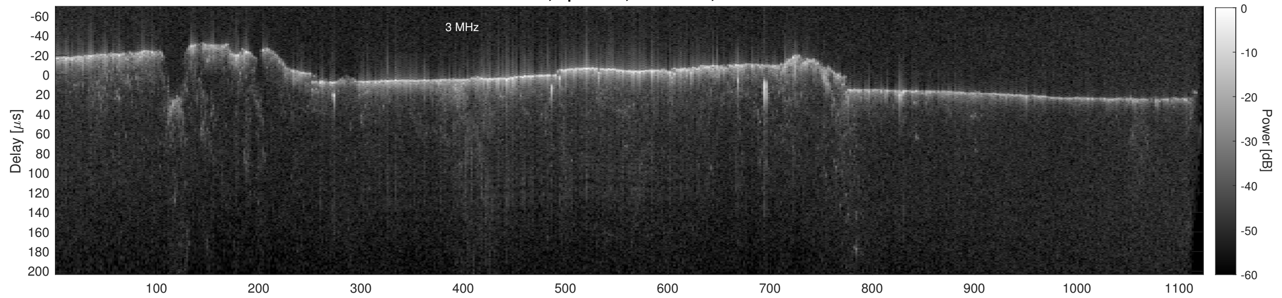
Orbit 14315, Cluttergram
