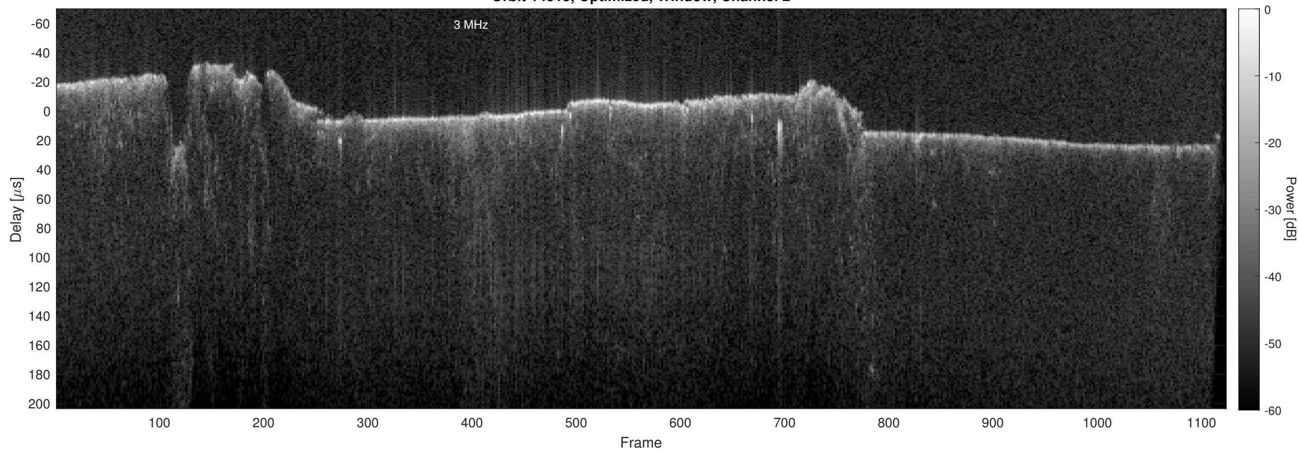
Orbit 14315, Optimized, Window, Channel 2
