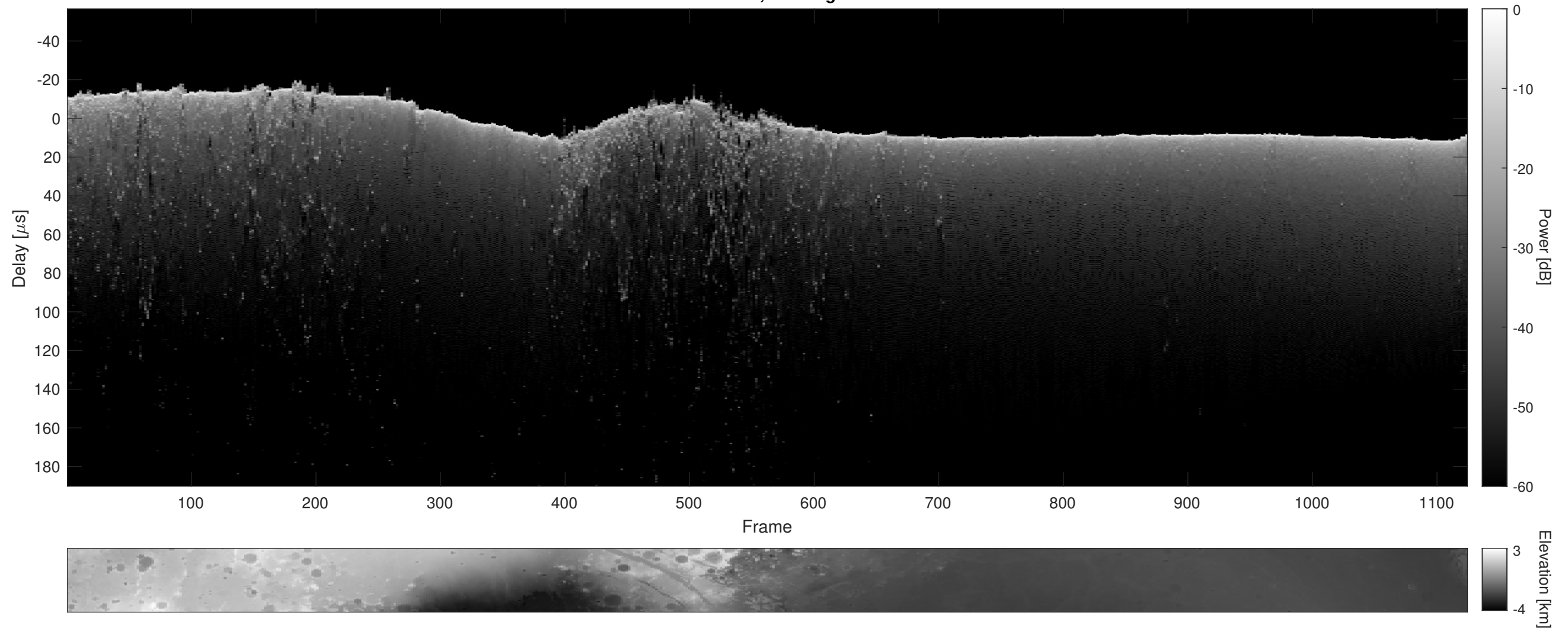
Orbit 14317, Cluttergram
