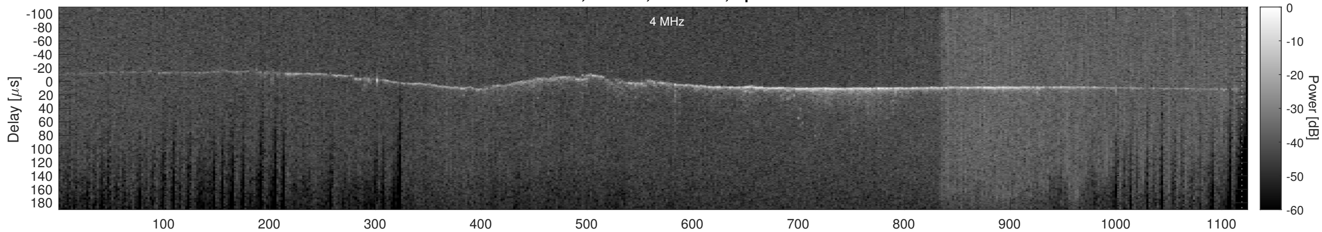
Orbit 14317, Cluttergram
