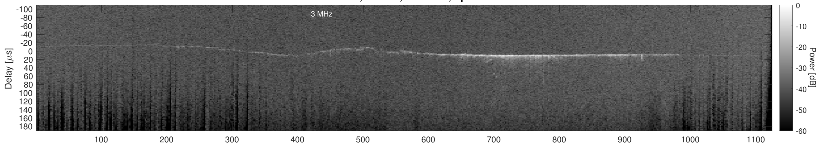
Orbit 14317, Cluttergram
