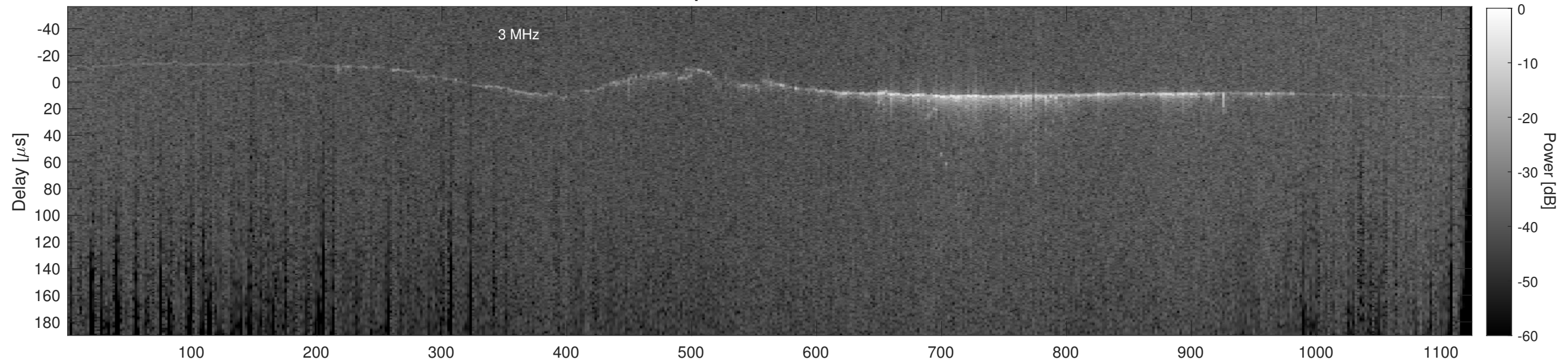
Orbit 14317, Cluttergram
