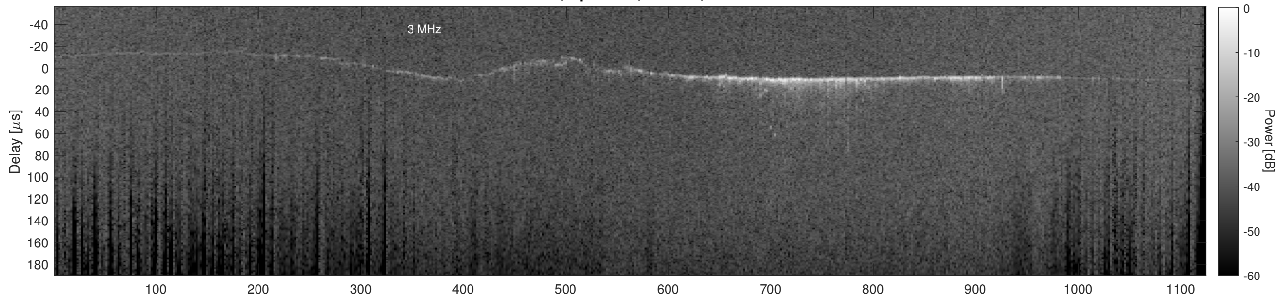
Orbit 14317, Cluttergram
