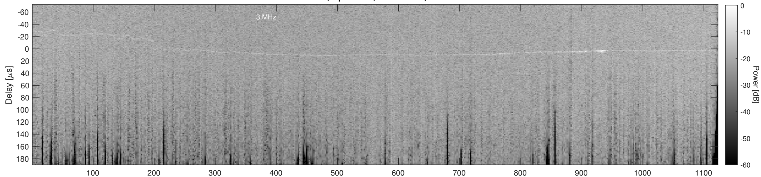
Orbit 14320, Cluttergram
