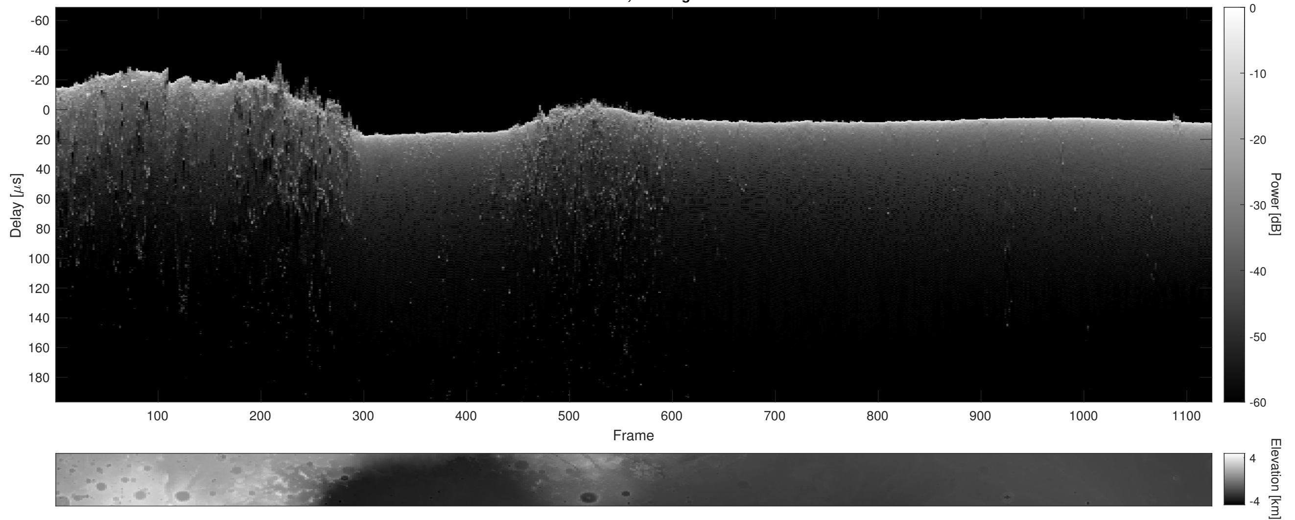
Orbit 14324, Cluttergram
