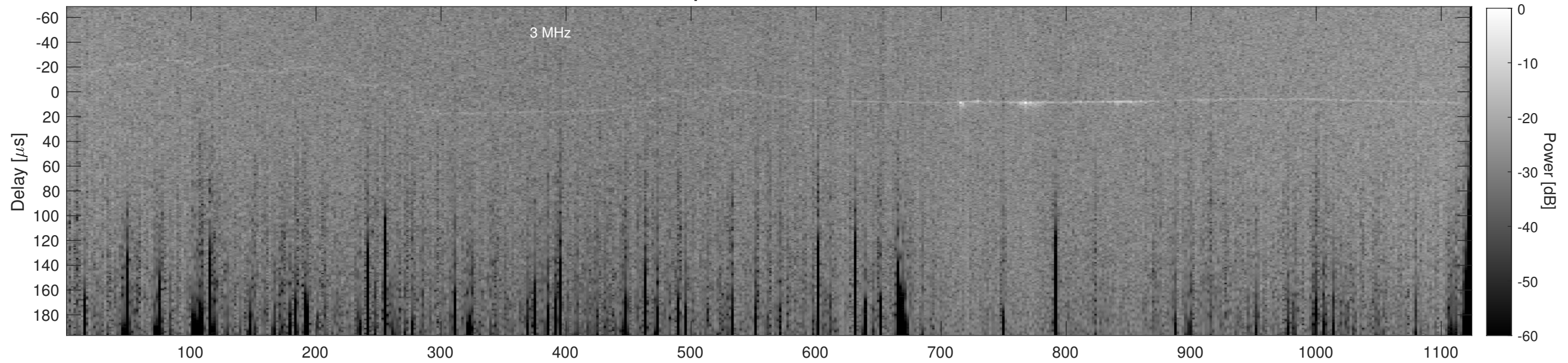
Orbit 14324, Cluttergram
