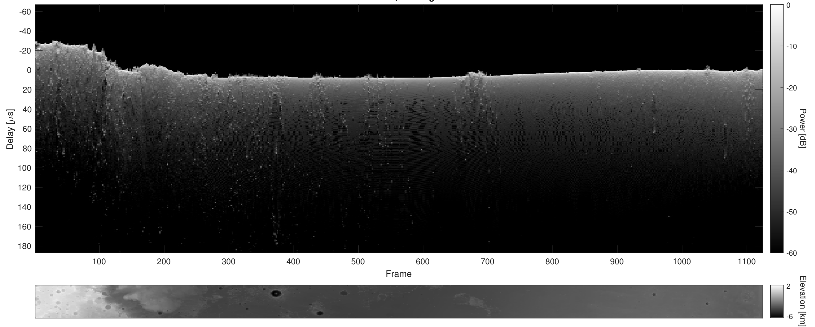
Orbit 14330, Cluttergram
