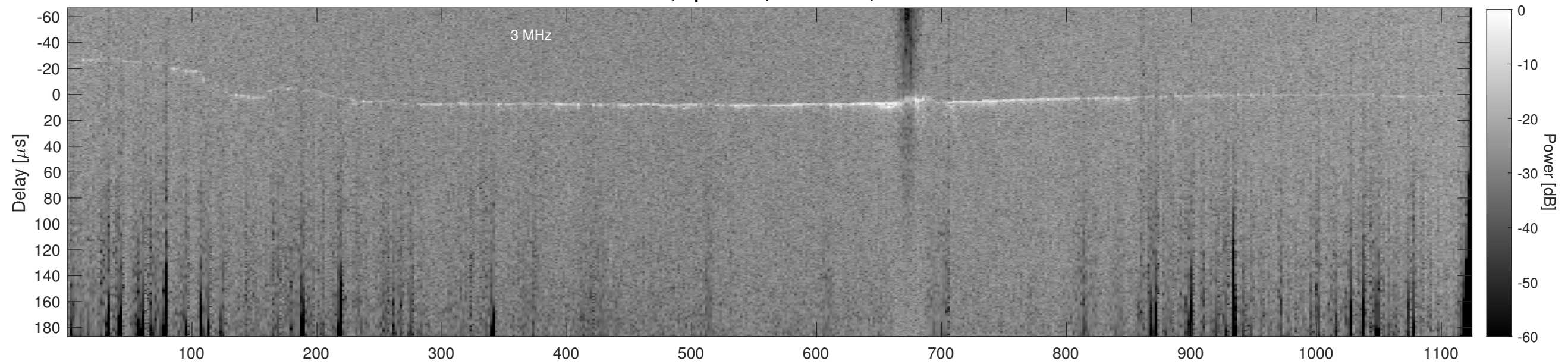
Orbit 14330, Cluttergram
