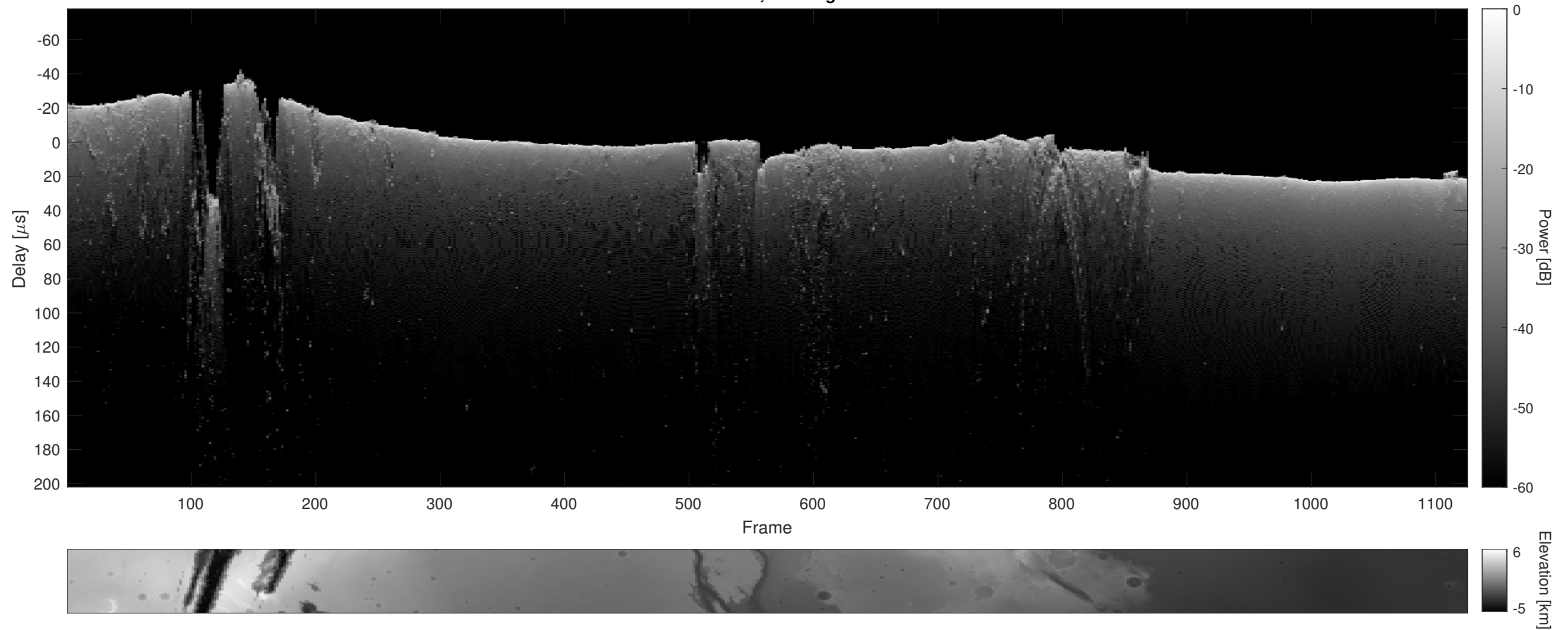
Orbit 14336, Cluttergram
