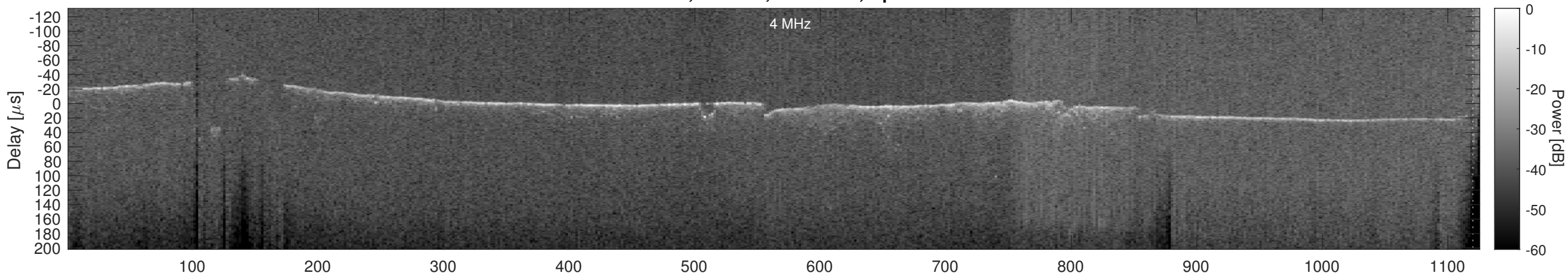
Orbit 14336, Cluttergram
