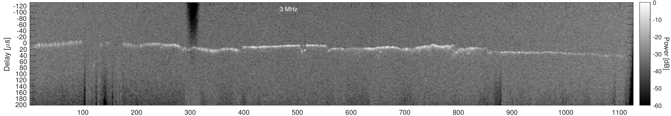
Orbit 14336, Window, Channel 2, Chapman
