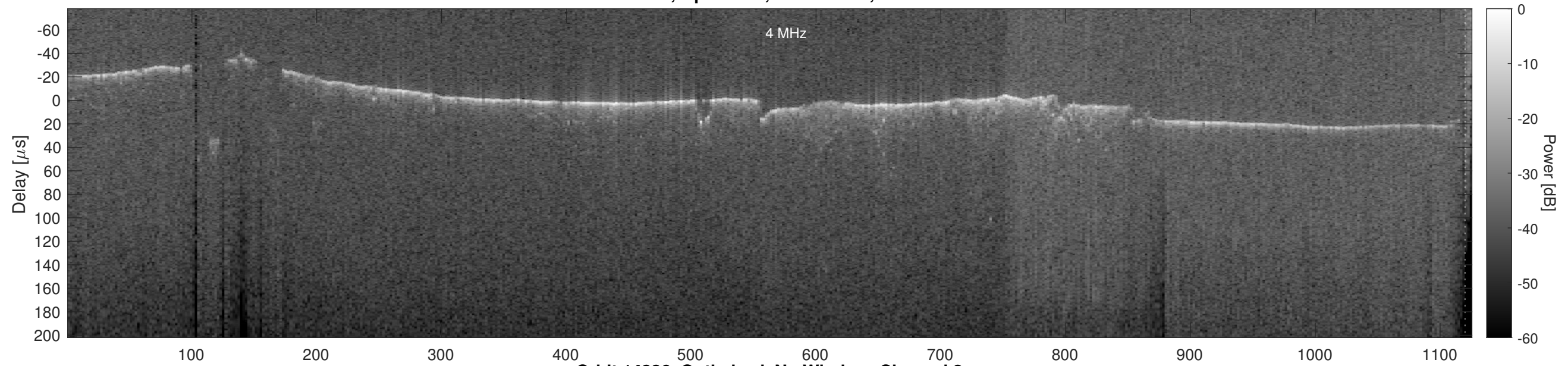
Orbit 14336, Optimized, No Window, Channel 2
