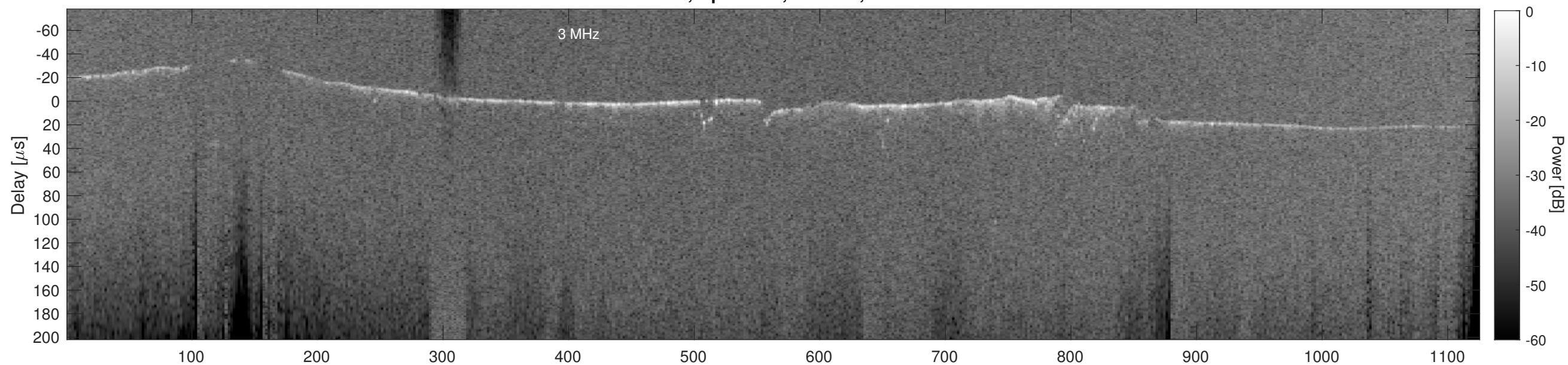
Orbit 14336, Cluttergram
