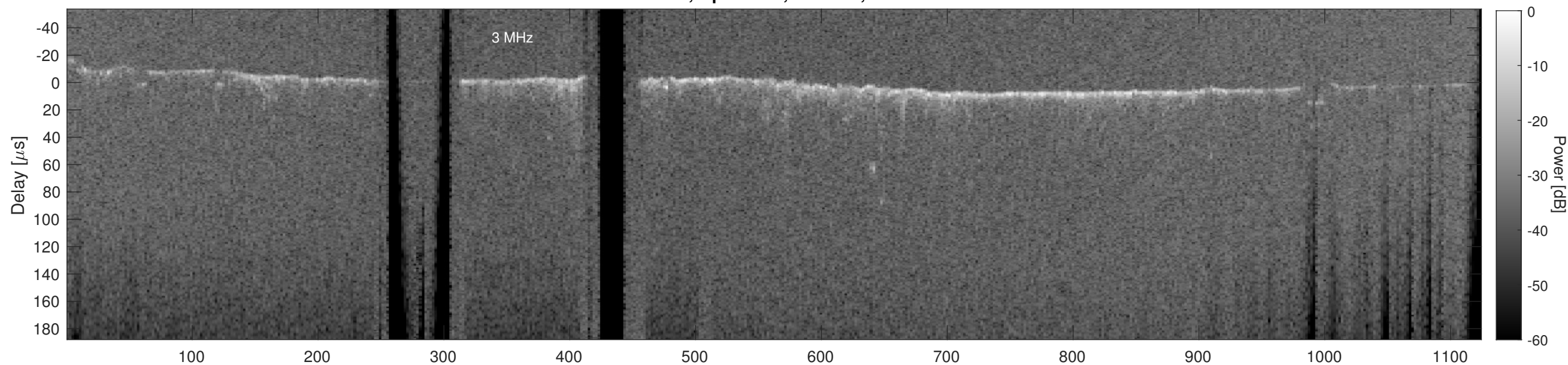
Orbit 14339, Cluttergram
