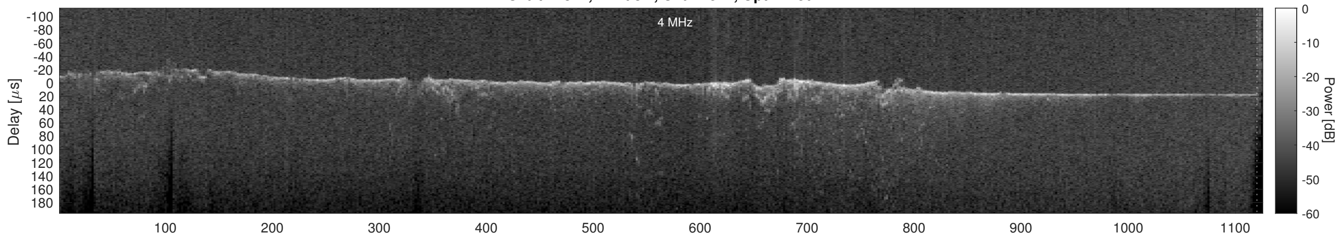
Orbit 14342, Cluttergram
