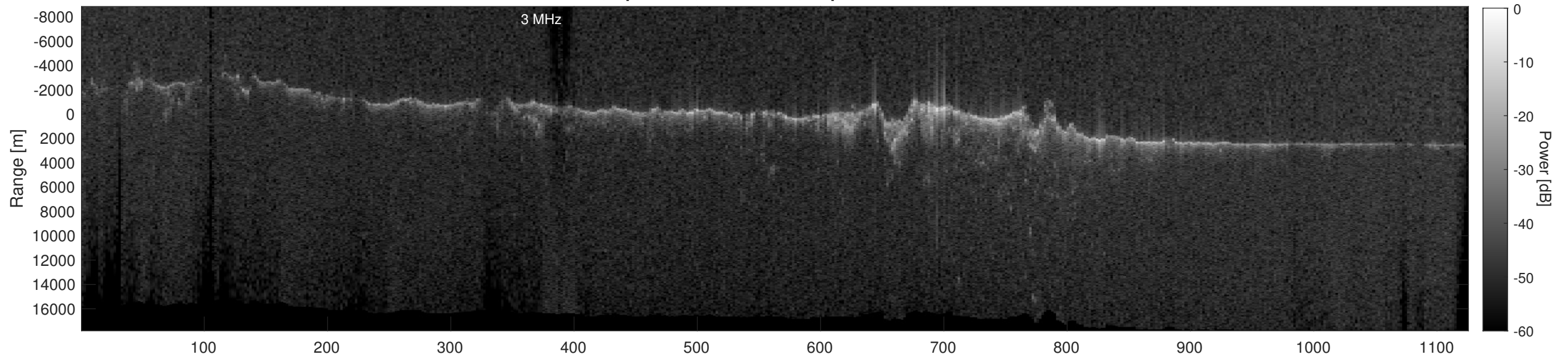
Orbit 14342, Depth-Corrected Cluttergram
