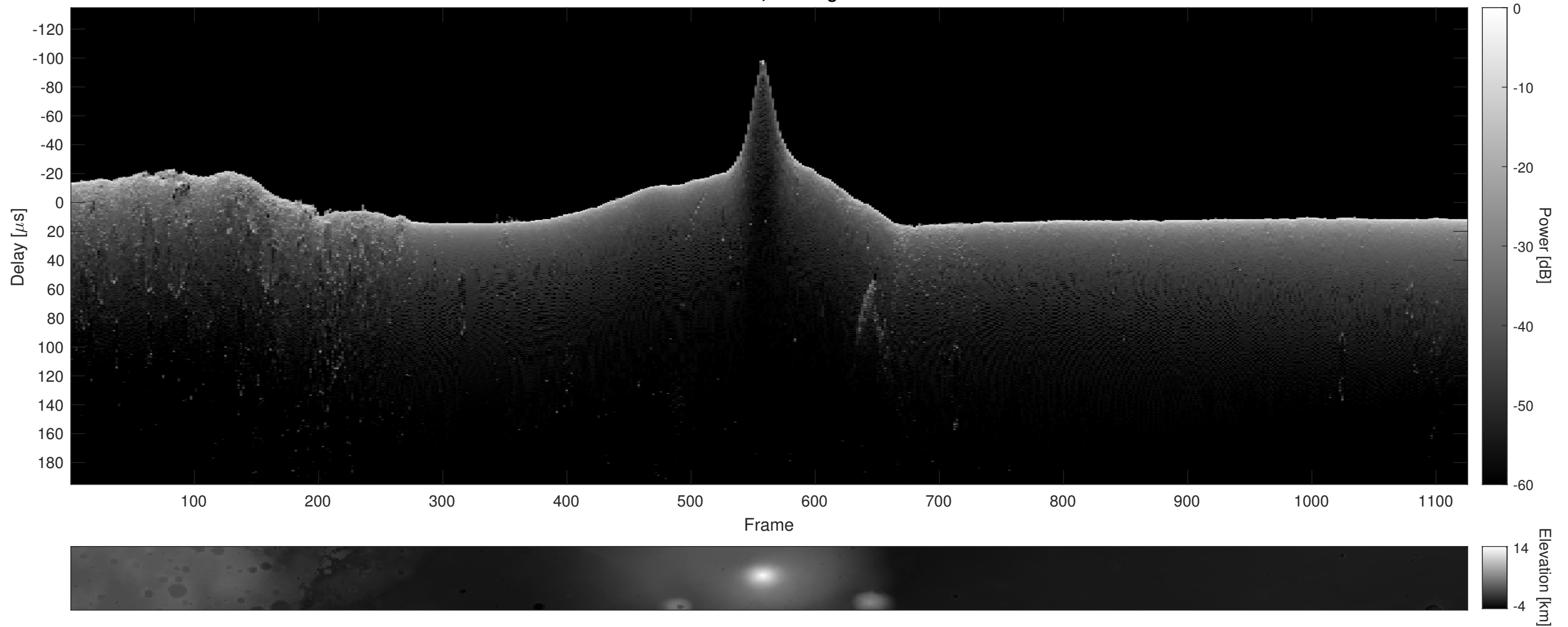
Orbit 14348, Cluttergram
