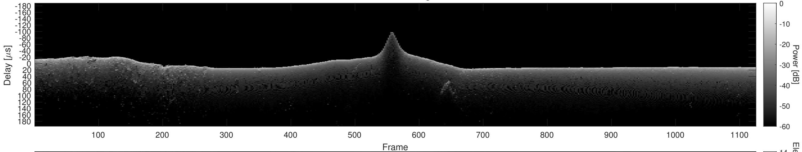
Orbit 14348, Cluttergram
