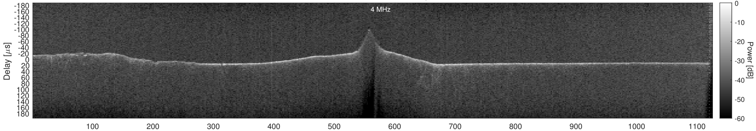
Orbit 14348, Cluttergram
