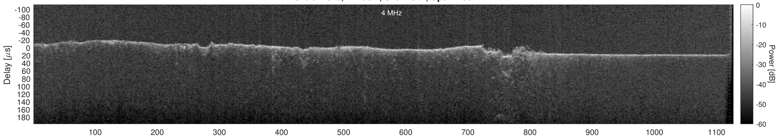
Orbit 14349, Cluttergram
