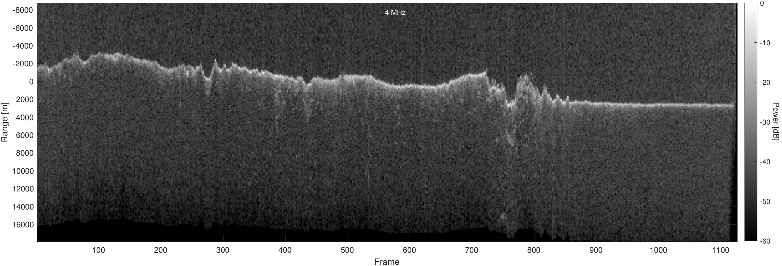
Orbit 14349, Optimized, Window, Depth-Corrected, Channel 2
