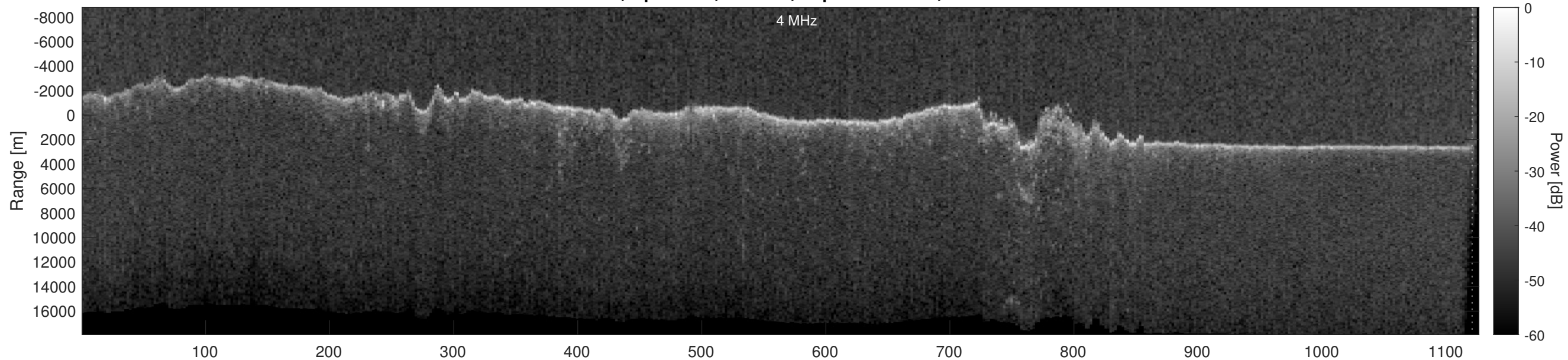
Orbit 14349, Optimized, Window, Depth-Corrected, Channel 2
