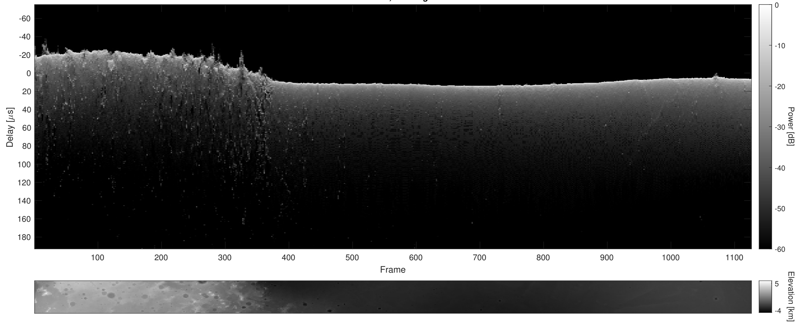
Orbit 14352, Cluttergram
