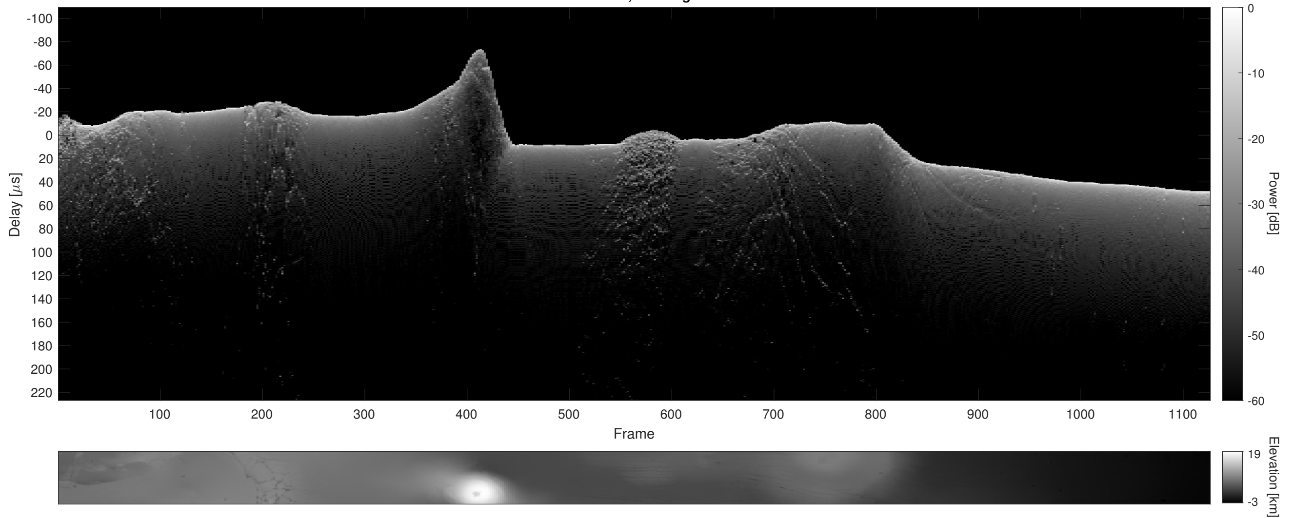
Orbit 14354, Cluttergram
