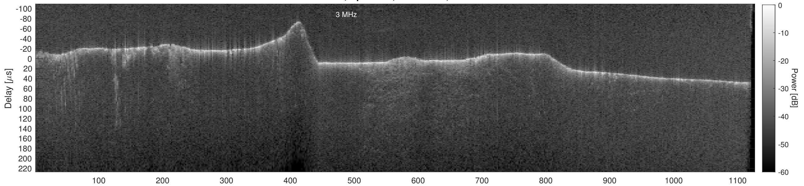
Orbit 14354, Cluttergram
