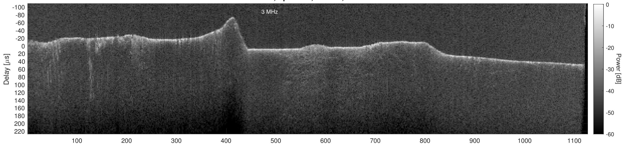
Orbit 14354, Cluttergram
