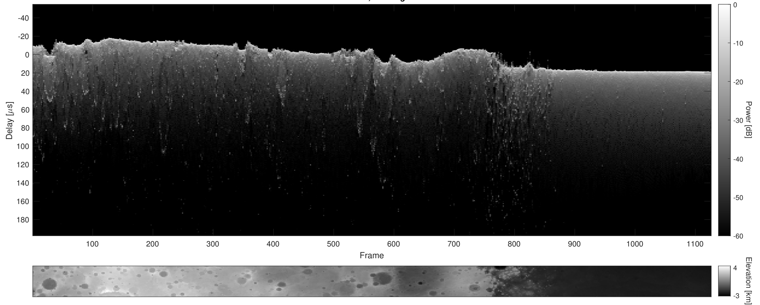
Orbit 14356, Cluttergram
