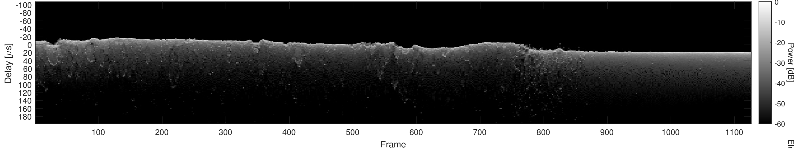
Orbit 14356, Cluttergram
