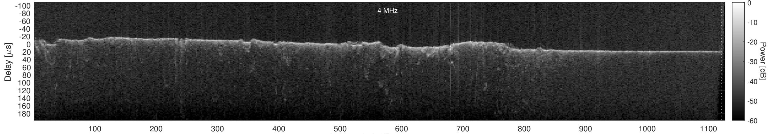
Orbit 14356, Cluttergram
