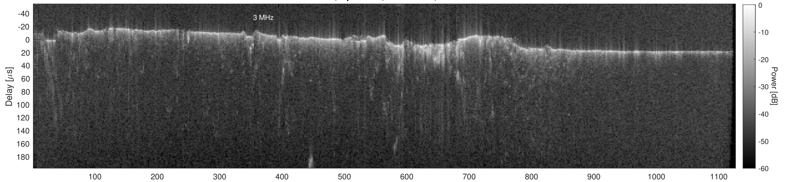
Orbit 14356, Cluttergram
