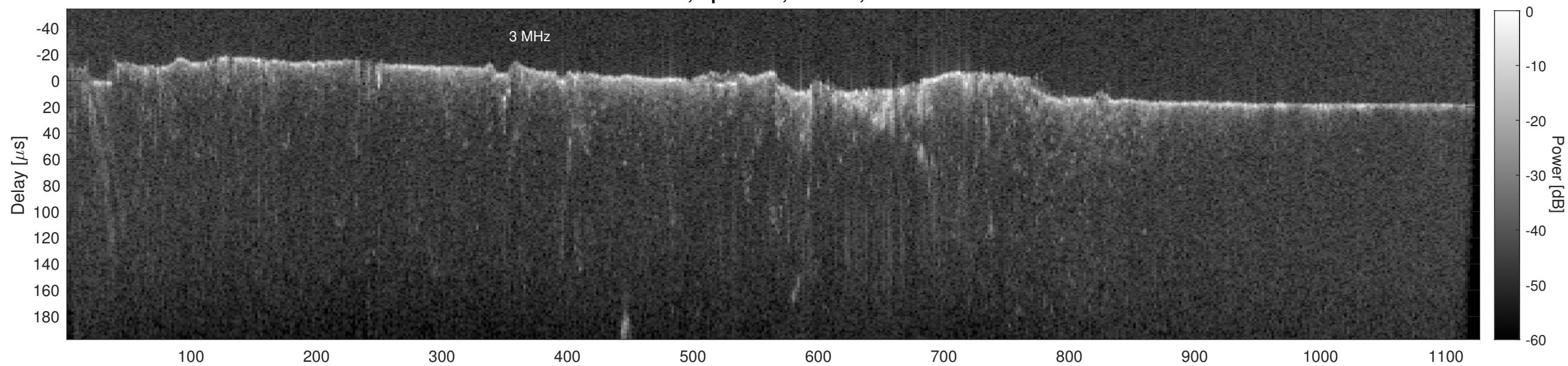
Orbit 14356, Cluttergram
