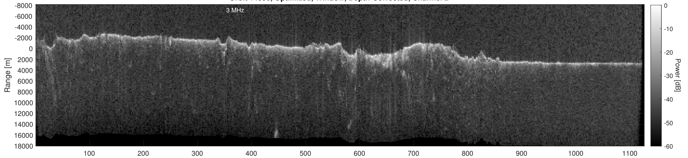
Orbit 14356, Depth-Corrected Cluttergram
