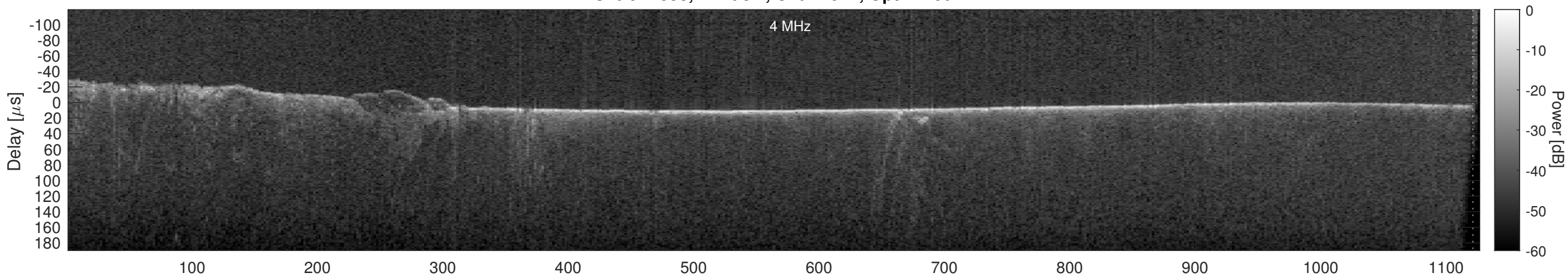
Orbit 14358, Cluttergram
