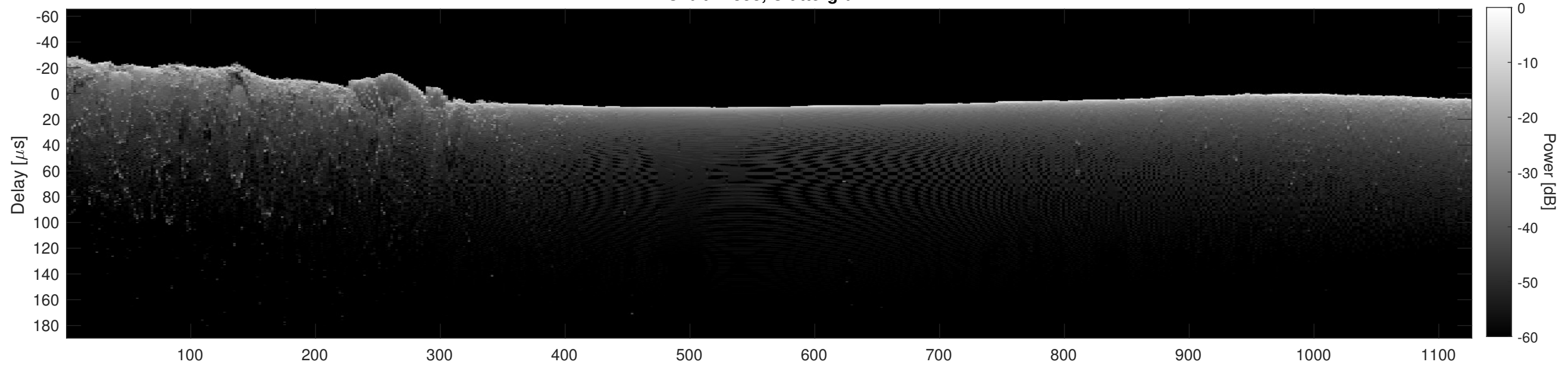
Orbit 14358, Cluttergram
