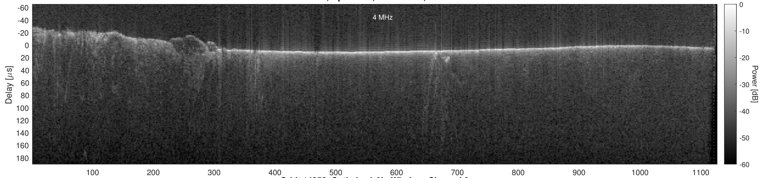
Orbit 14358, Optimized, No Window, Channel 2
