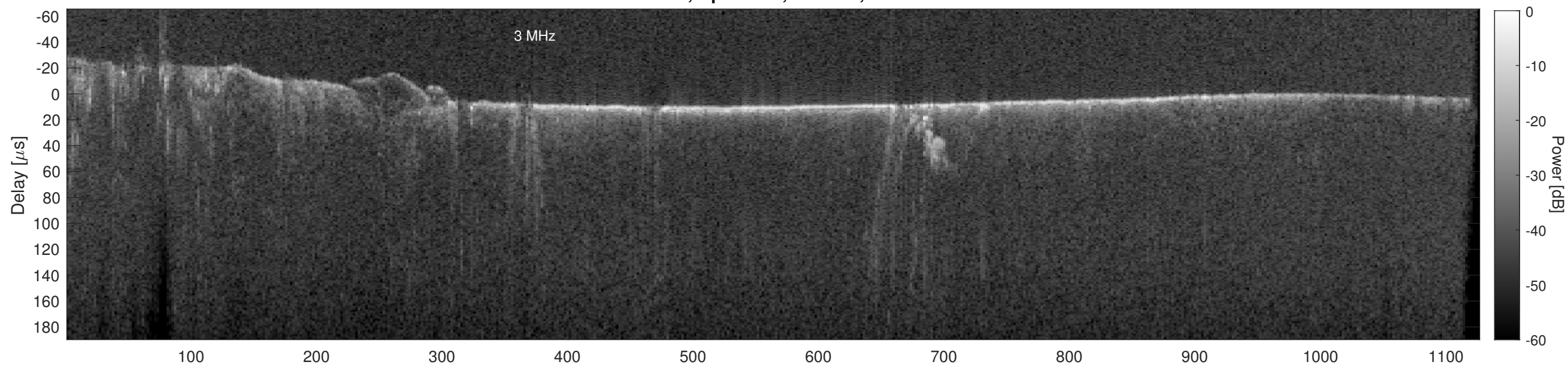
Orbit 14358, Cluttergram
